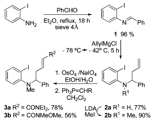
Scheme 1. Synthesis of N -Alkenyl Substituted o -Iodoanilines 2a,b and 3a,b
